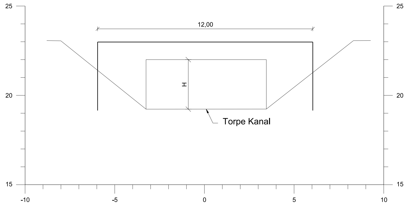
SECTION B-B 1:100 St. 78+484.557
