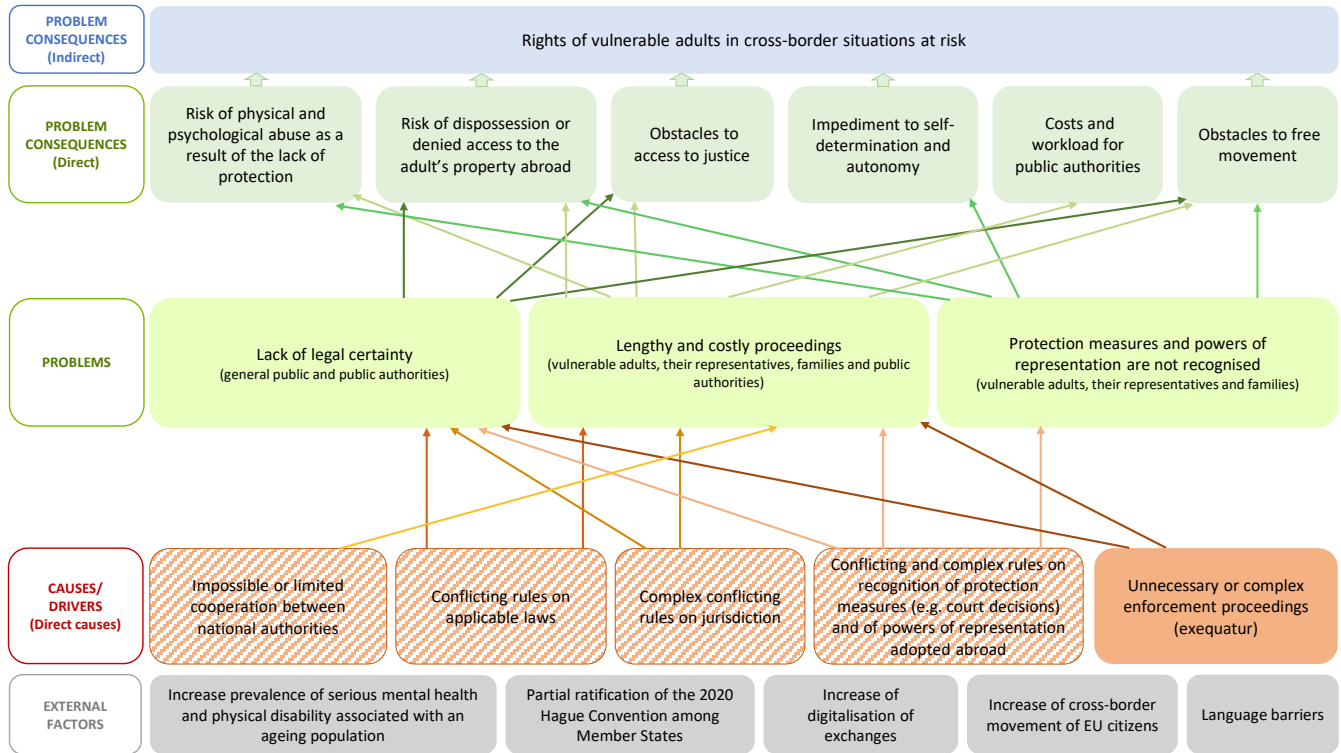
Figure 1: Problem Tree
